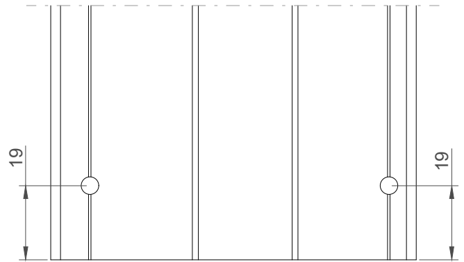
Drilling dimensions 38 0001
